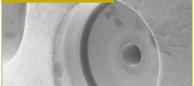
Step hole by milling and spray hole by EDM
